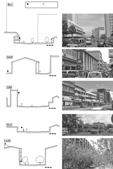
Fig 2: Positioning of measurement equipment within urban canyons.
