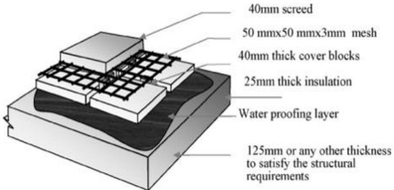
Figure 11: The system with continuous concrete strips (Halwatura & Jayasinghe, 2008)
